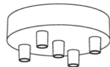
KRM575FGOTERM 5 hole ø 120mm H 25mm
